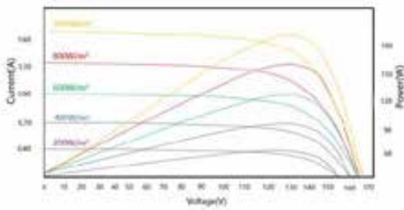
COM-Z2 at different light intensities
