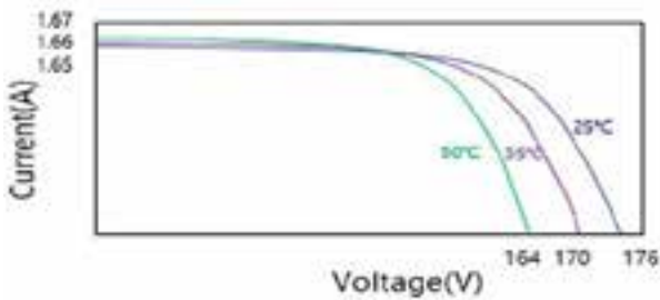
COM-Z2 at different temperatures
